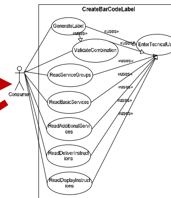
Use Case Model
